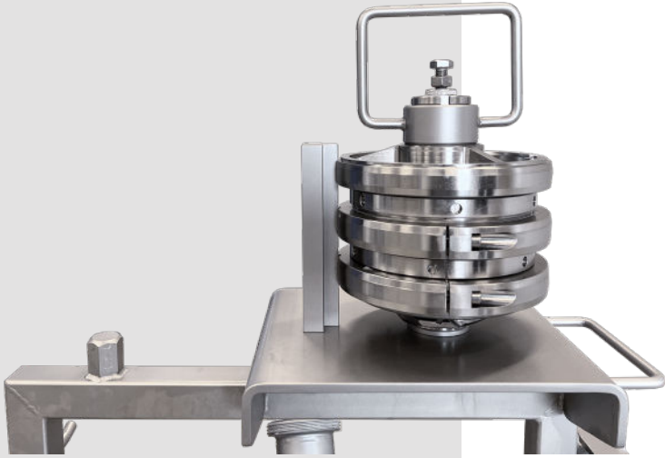
scanEmul 175 knife cassette shown assembled.
